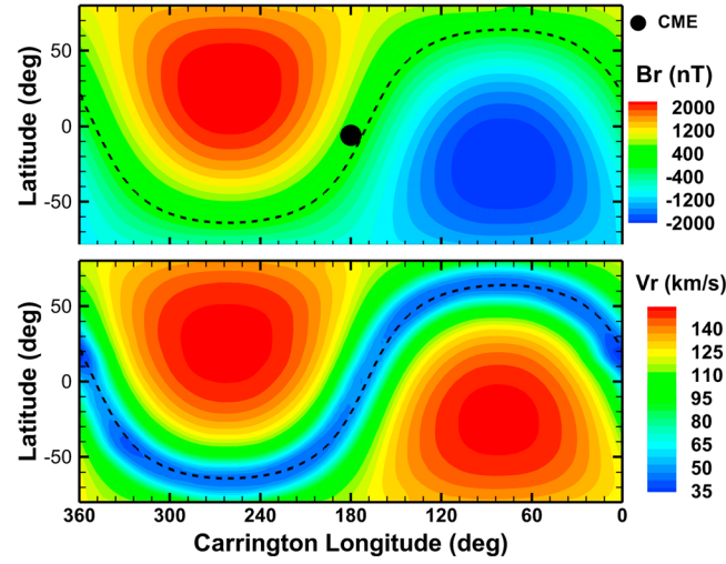
Figure 3. The steady state distribution of radial component of (top) magnetic field and (bottom) velocity at 5 R_{\odot} . The dashed lines in each panel show the location of B_r = 0 .
