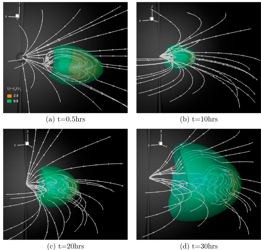
Figure 9. Three-dimensional view of the relative density ( (\rho - \rho_0)/\rho_0 ) distribution at t = 0.5, 10, 20 , and 30 h. The color code in the panels represents the two levels of isosurfaces of the relative density. The magnetic field topology is represented by the white magnetic field lines.
